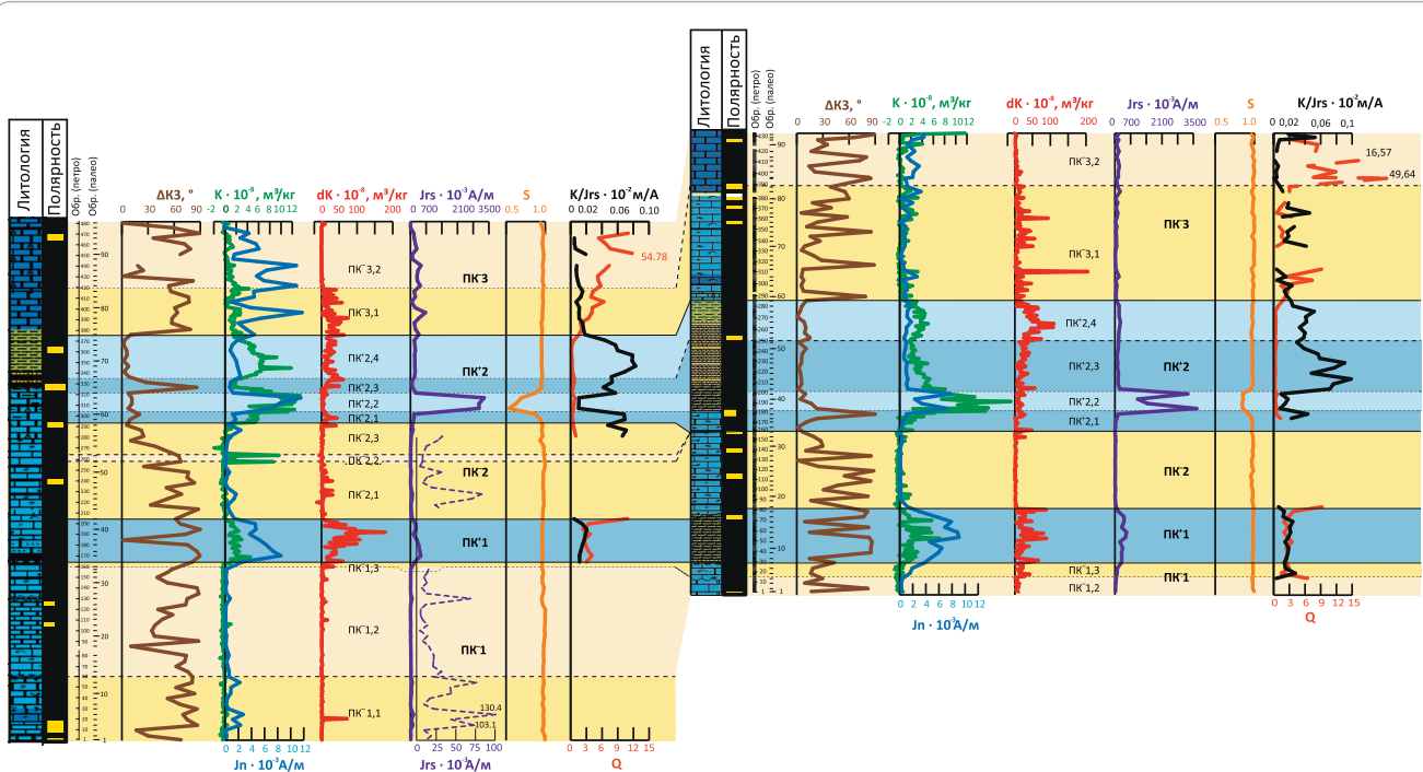
Fig. 7. Fragment of the correlation chart based on petromagnetic data for the Jurassic – Cretaceous boundary interval exposed in the wells
