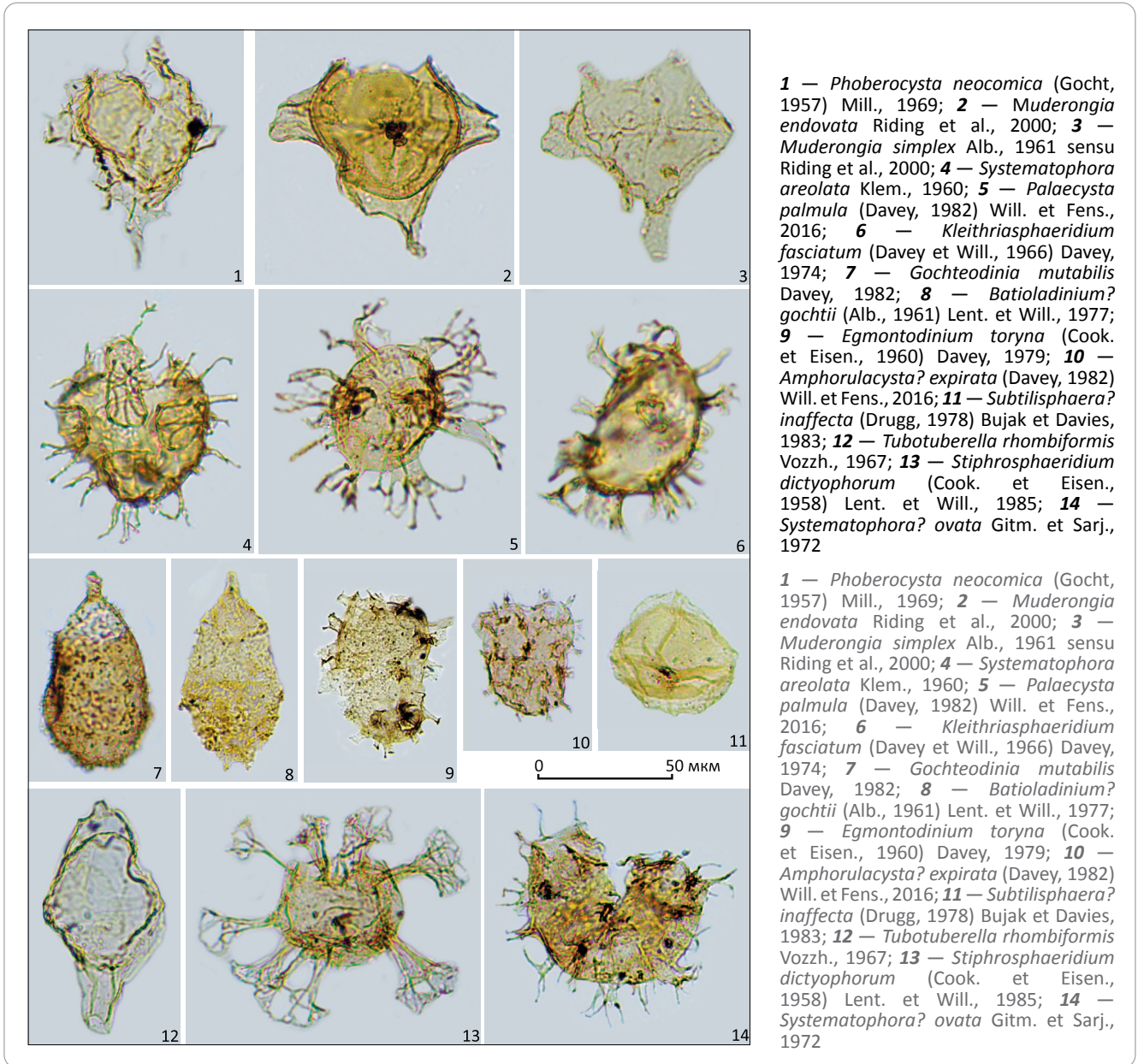
Fig. 6. Dinocysts of the Tithonian-Berriasian deposits in the North Caspian region
